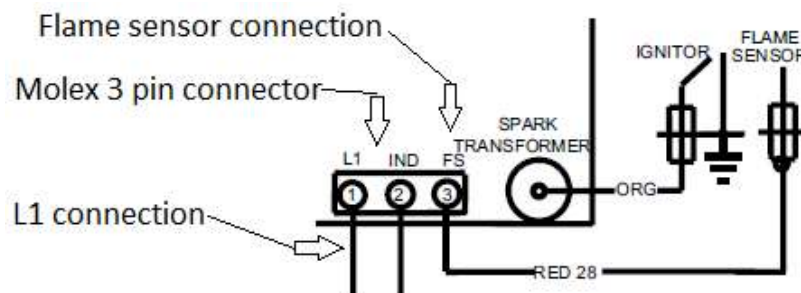
Single Stage Gas – Line Voltage Connections
